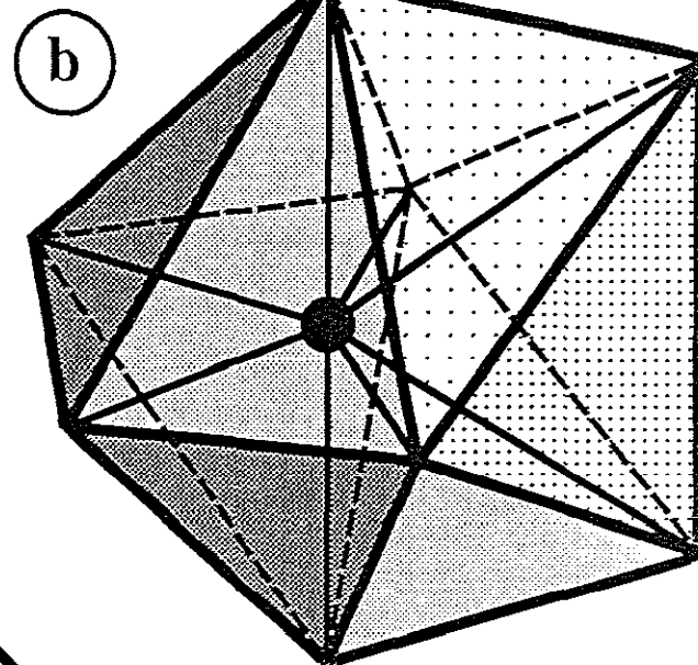
BISDISPHENOID CN 8
