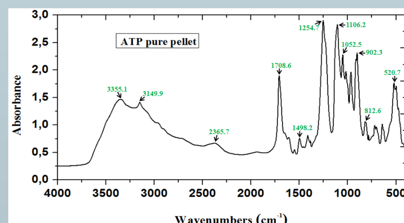
Fig.2 Experimental IR spectrum for ATP molecule.
