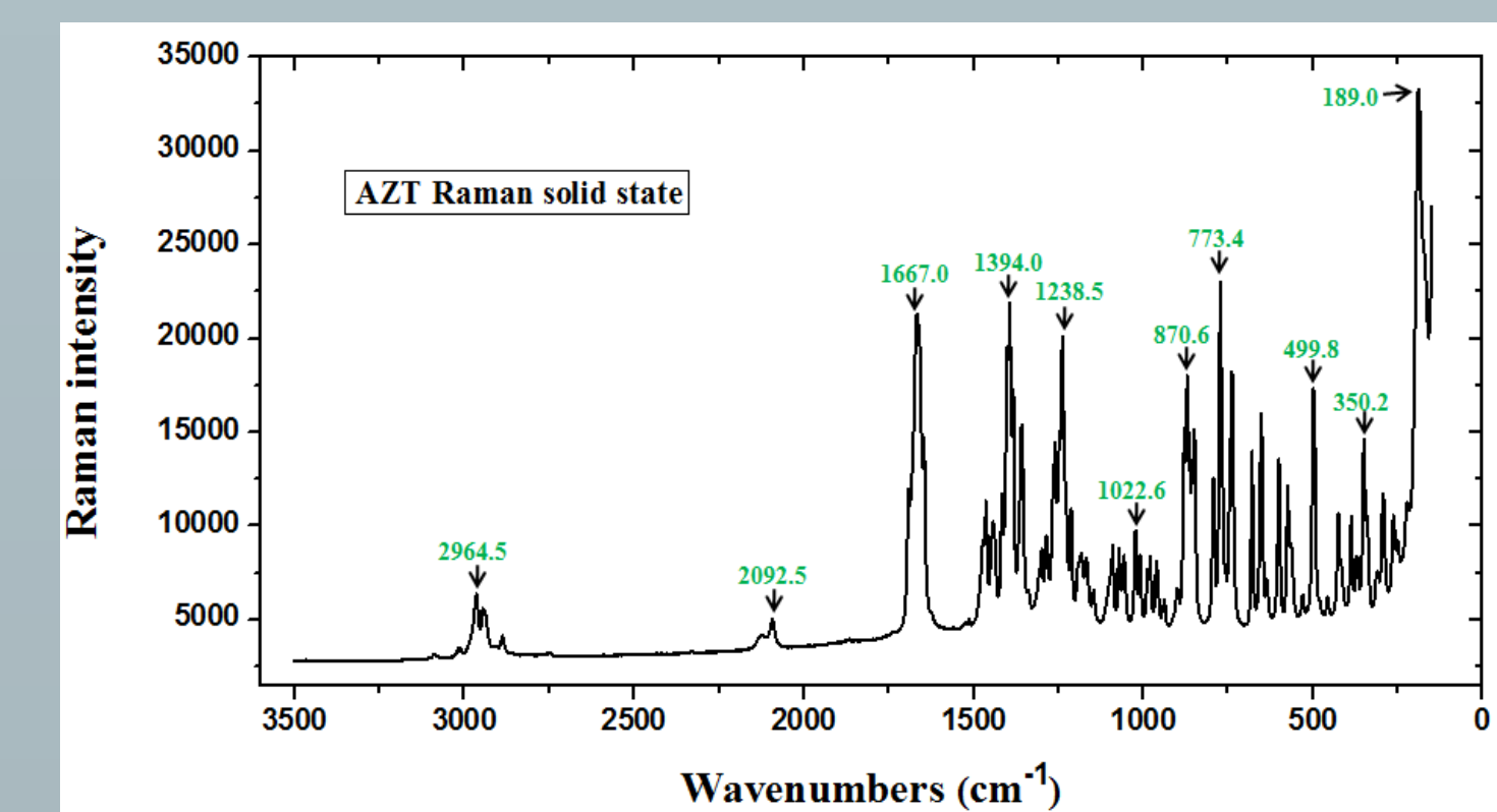
Fig.6 Experimental Raman spectrum for AZT molecule.
