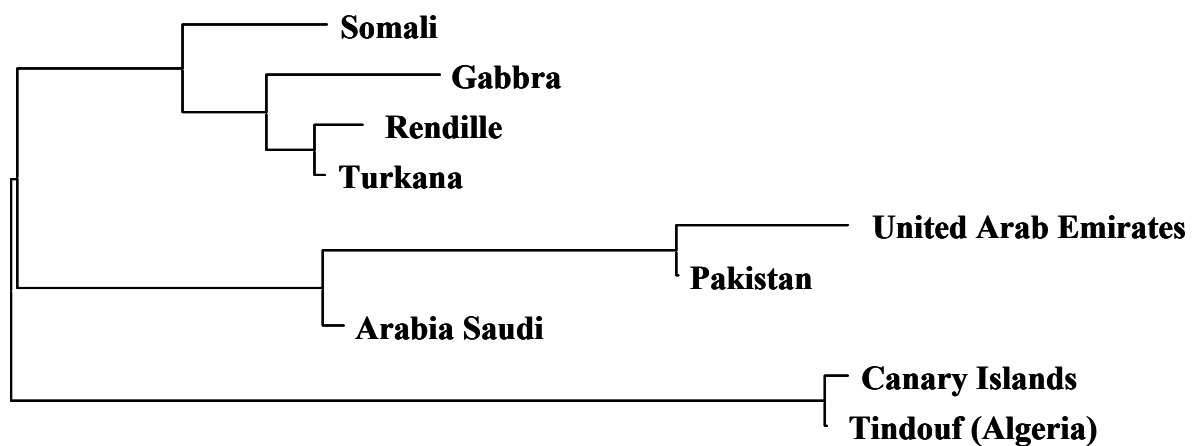
Figure 3. Neighbor-Joining tree of genetic distances based on estimated membership coefficients q_k(i) of population i for cluster k as in [13].
