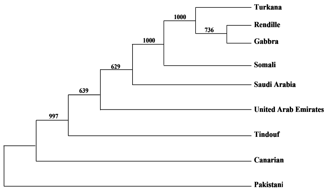
Figure 1. Consensus Neighbor-Joining tree based on the F_{ST} distances. The numbers on the branches indicate bootstrap values (the number of times the partition of the populations into the two sets separated by that branch occurred among the trees, out of 1,000 trees).
