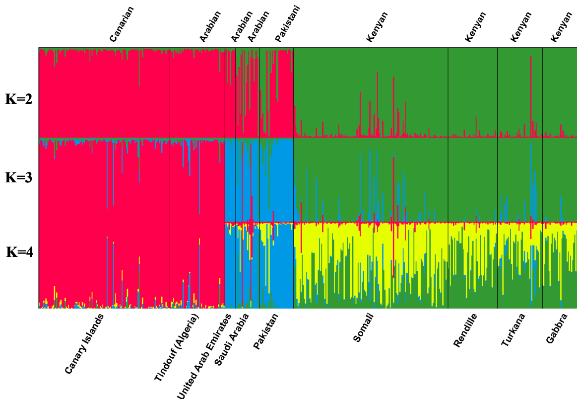
Figure 2. Stacked vertical line plots of the estimated membership fractions of each individual analyzed for each of the k inferred clusters with k from 2 to 4. Individuals are grouped by population.
